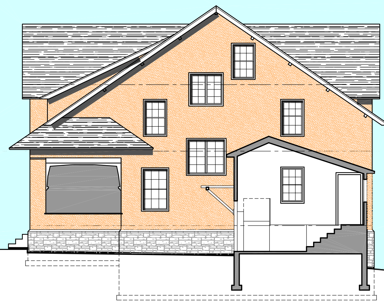
SECTION THROUGH NEW ENTRY
